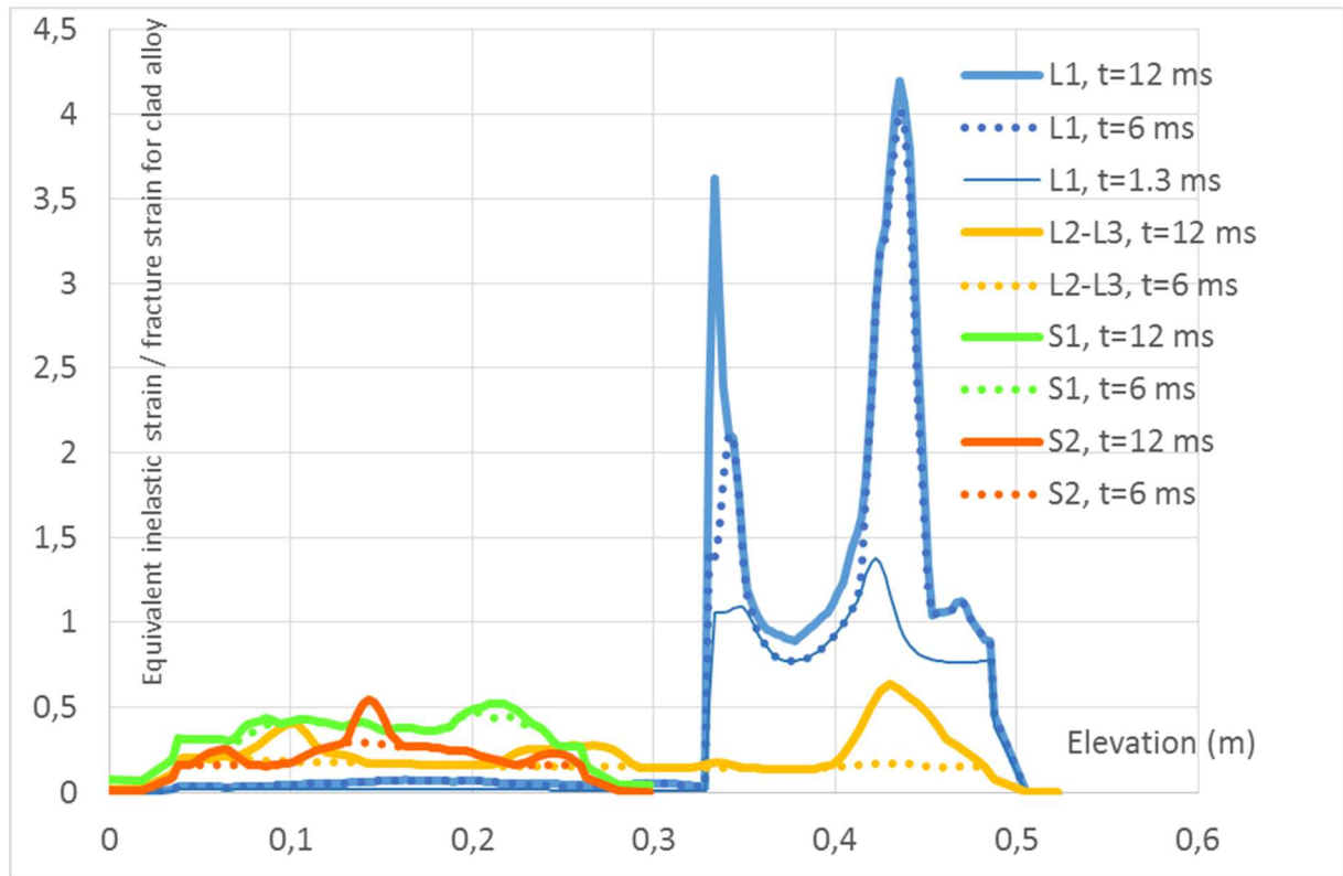
FIG. 6 – Equivalent inelastic strain normalized by the fracture strain of the clad as a function of the elevation at time 1.3, 6 and 12 ms. Case of clad alloy 1.
