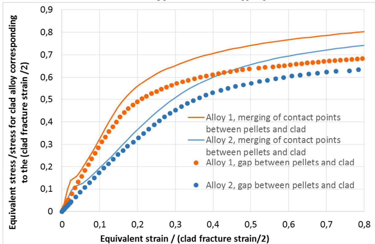
FIG. 2 – Equivalent stress-strain law obtained from four points bending calculations of rod segments with different clad alloys and clad-pellets boundary conditions (strains normalized to half of the fracture strains of the clad alloys and strength normalised to strength values at these strains).
