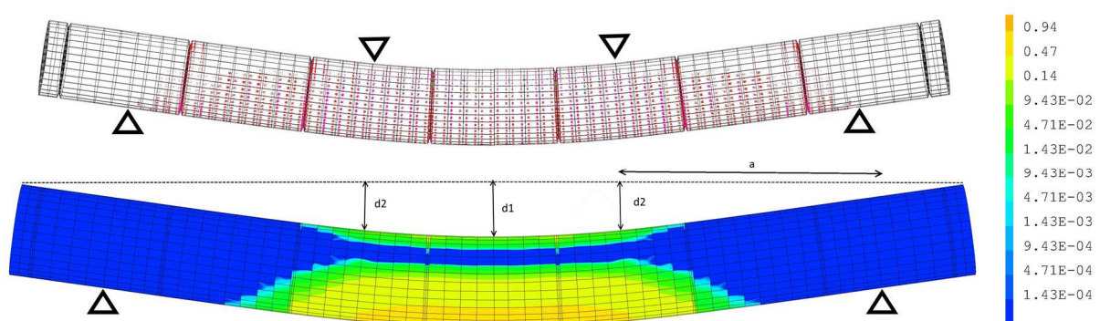
FIG. 1 – Cracks openings (top) in the pellets displayed in red and inelastic strain (bottom) in the clad (normalized to the fracture strain) resulting from four points bending of a rod segment. The support pins and loading pins are displayed as triangles.
