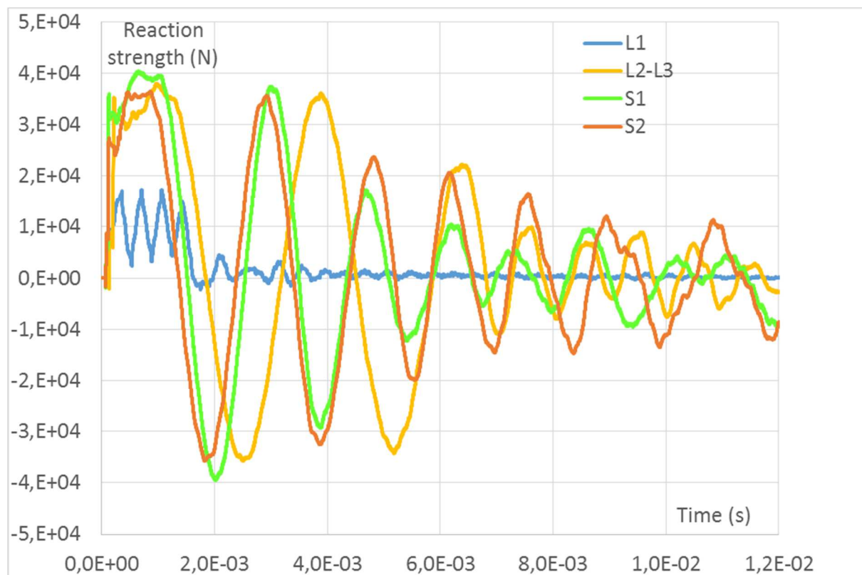
FIG. 4 – Variation of the calculated reaction strength at the lower point of the specimen as a function of the time. Case of clad alloy 1.
