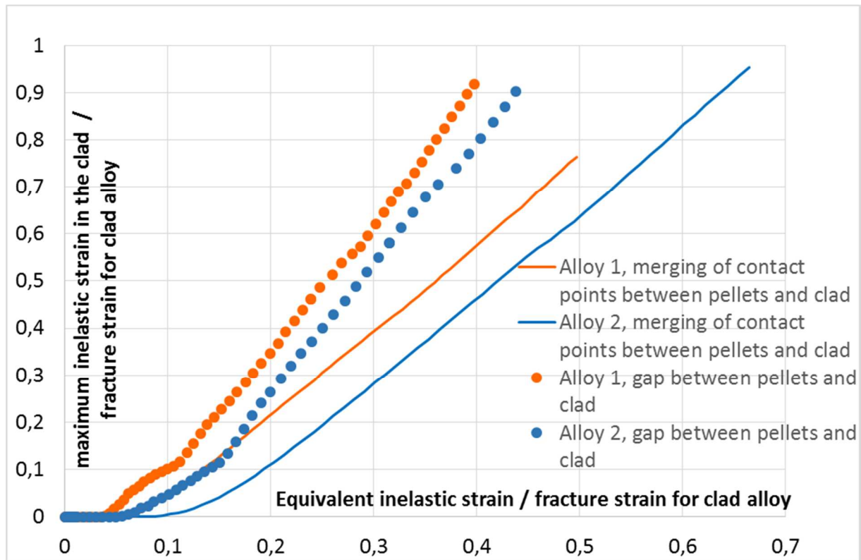
FIG. 3 – Maximum inelastic strain in the clad as a function of the equivalent inelastic strain calculated from four points bending of rods with different clad alloys and clad-pellets boundary conditions. Strains are normalized to the fracture strains of the clad.
