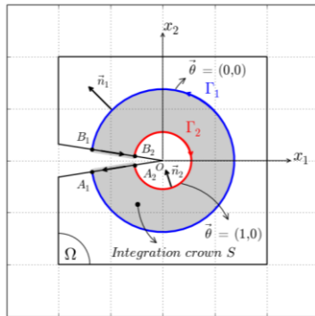
Fig. 1: Description integral domain of J and G θ
