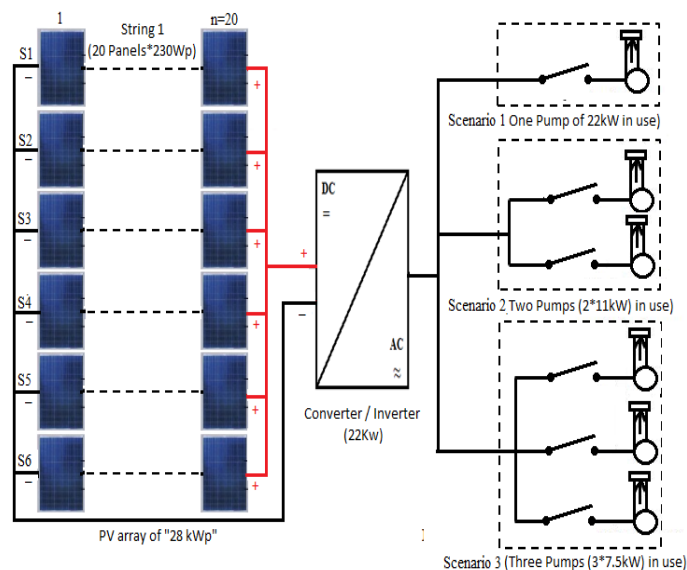
Figure.1 Three proposed scenarios of photovoltaic water pumping systems.
