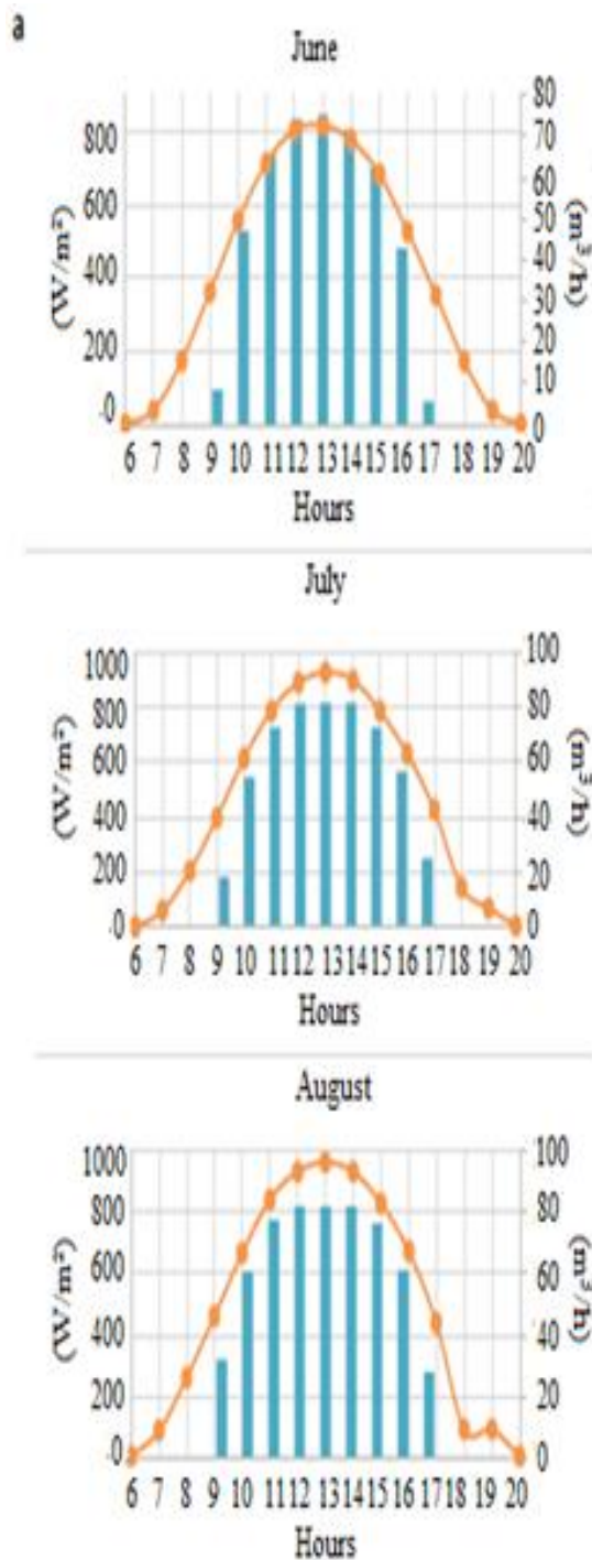
Figure. 2.a Average daily pumped water versus irradiance using one large pump of (22 kW).
