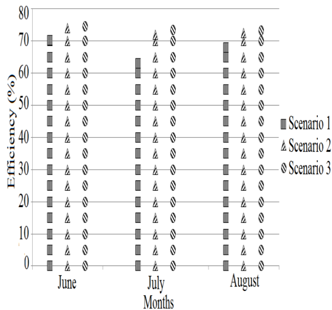
Figure.4 Pump powers management vs hydraulic efficiencies (Three scenarios).
