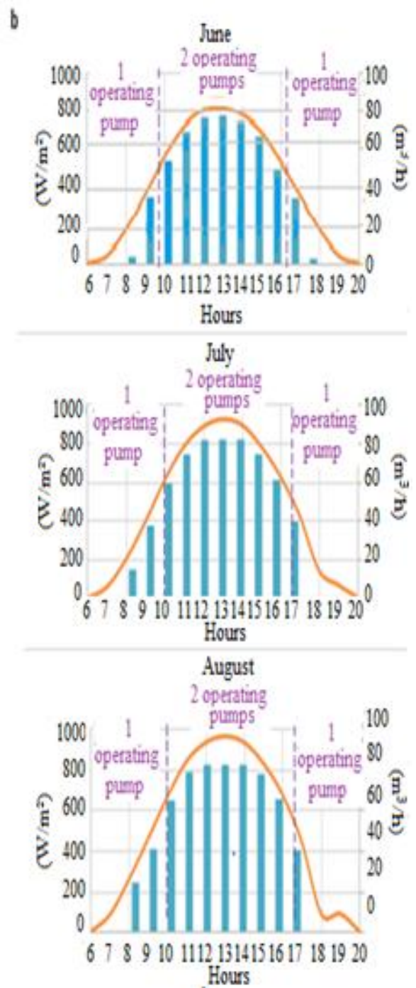
Figure. 2.b Average daily pumped water versus irradiance using two small pumps (2*11 kW).
