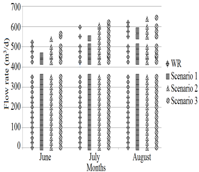
Figure.3 Average daily water requirements and pumped volumes.
