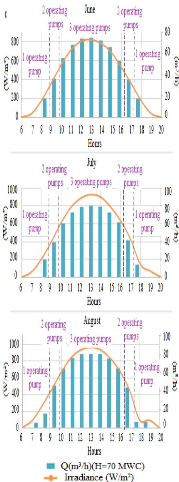
Figure. 2.c Average daily pumped water versus irradiance using three small pumps (3*7.5 kW).
