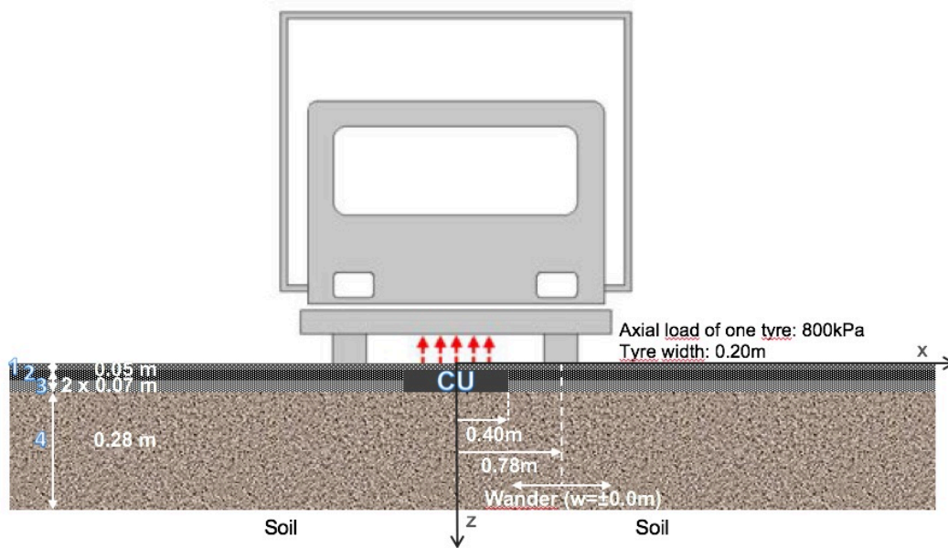
FIG. 1 - A half cross-sectional geometry of an eRoad with an inductive CU (After [9])
