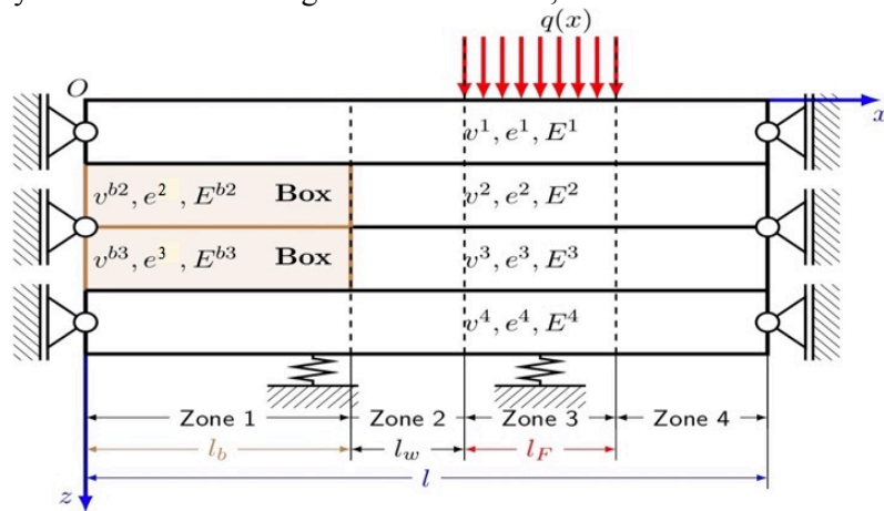
FIG. 2 - M4-5nW equivalent eRoad model of half the cross-sectional geometry (After [7])
