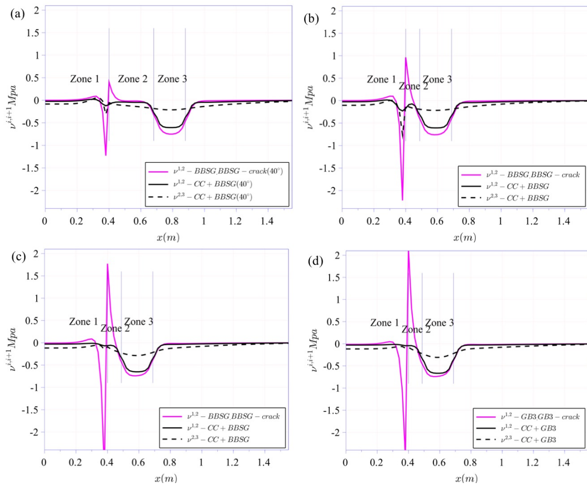
FIG. 3 - Interfacial normal stress comparison between the various cases: (a) BBSG ( 40^\circ, E^3 = 1000\text{MPa} , w=0 ); (b) BBSG ( 40^\circ , w=-0.2 ); (c) BBSG ( 15^\circ\text{C} , w=-0.2 ); (d) GB3 ( 15^\circ\text{C} , w=-0.2 )
