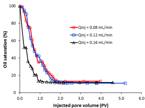
Figure 11: Averaged oil saturation vs injected PV for the model of packed sand.
