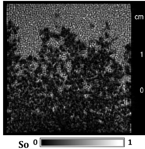
Figure 3: MRI vertical slice of a stack of polystyrene beads contained in a PVC tube and initially saturated with oil. The aqueous solution of \text{MnCl}_2 is injected from the bottom with a flow rate of 0.12 mL/min. The image is obtained after 3h45 of water injection. Water saturated regions appear in black and those saturated with oil in white.
