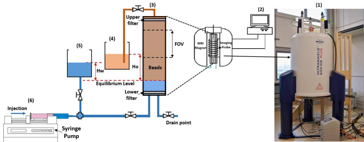
Figure 1: Experimental setup: (1) 600 MHz NMR system; (2) Computer for data process; (3) Porous media sample; (4) Oil tank; (5) Water tank; (6) Water injection pump.
