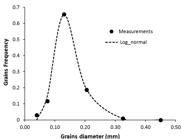
Figure 2: Sand Grain frequency vs grain size matching with Log-normal function.
