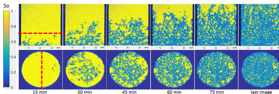
Figure 4: Consecutive MRI images of the water–oil displacement in the model of polystyrene beads with the injection flow rate of 0.12 mL/min. The oil is yellow and the water is light blue. The acquisition of MRI signal was made each 15 minutes and shown here from the first water appearance in FOV. The dotted line on the first vertical section indicates the position of the horizontal sections (and vice-versa for the horizontal section below).
