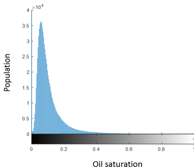
Figure 10: Histogram of residual oil distribution corresponding to its population in sand beads model ( Q_{inj} 0.12 mL/min).
