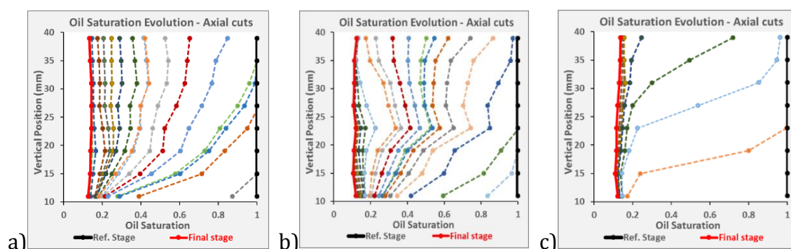
Figure 9: Oil saturation distribution in the packed sand model at different injection flow rates: (a) 0.08 mL/min, (b) 0.12 mL/min and (c) 0.16 mL/min.
