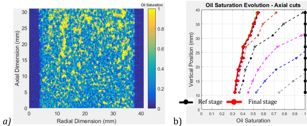
Figure 5: Residual oil saturation image in a vertical section (a) for the displacement process after the injection of 3.5 PV of the displacing fluid. Time evolution of oil saturation profiles deduced from the 8 axial sections (b).
